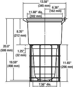
KSE Ballast Tank KG40 Optics Globe KAG40S Wire Guard
