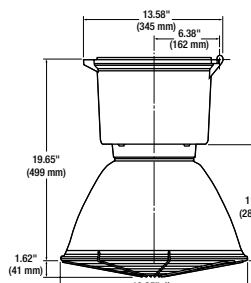
KSE Ballast Tank KER40 Enclosed Reflector KERG Wire Guard
